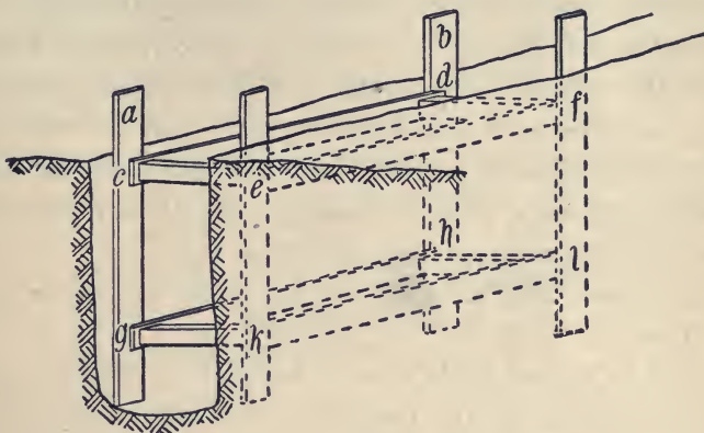
FIG. 13.—SKELETON SHEATHING.
